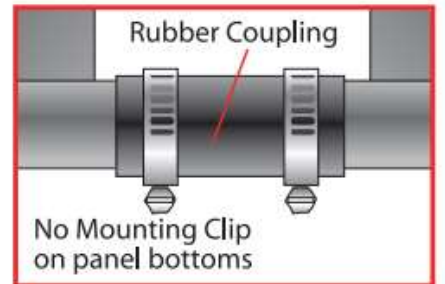
DETAIL D TOP VIEW
